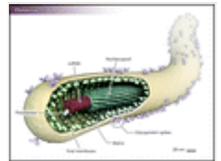
Structure of Ebolavirus.
