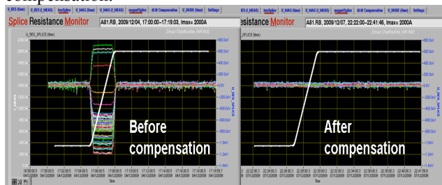
Fig 1: Busbar signals before and after compensation
