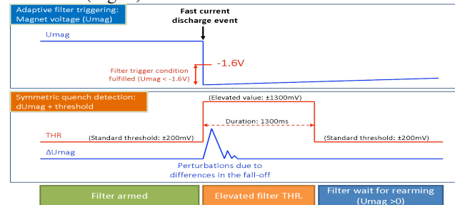
Fig 3: Symmetric quench adaptive filter logic
