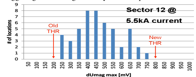
Fig 4: Statistics of perturbation voltage amplitudes
