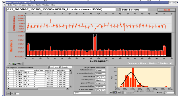
Fig 2: Splice mapping for quadrupoles in sector 12
